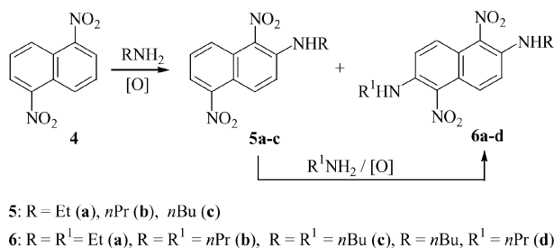
Scheme 3. Oxidative alkylamination of 1,5-dinitronaphthalene ( 4 ).
