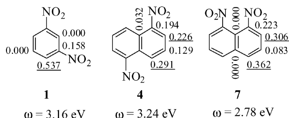
Figure 4. Calculated global electrophilicity values ( \omega , in eV) and local electrophilicity indices ( \omega_k , given at each ring atom, in eV).
