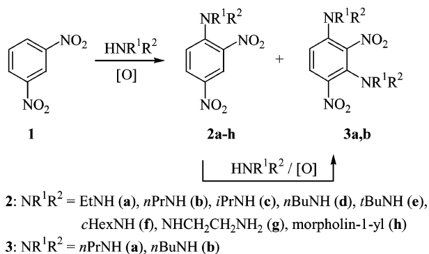
Scheme 2. Oxidative alkylamination of 1,3-dinitrobenzene ( 1 ).
