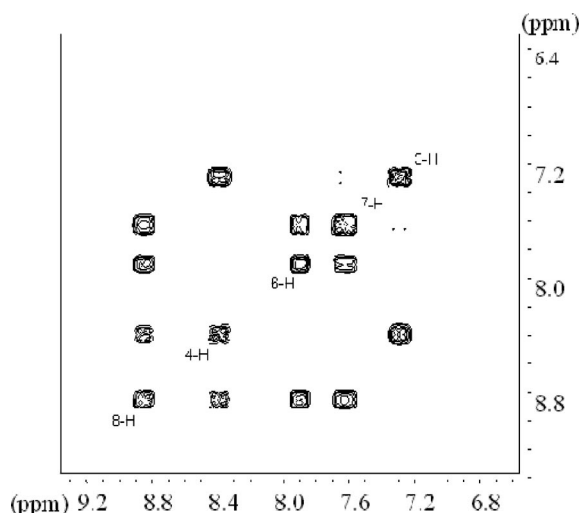
Figure 2. Fragment of the 1 H– 1 H COSY NMR spectrum of compound 5a (CDCl 3 ).
