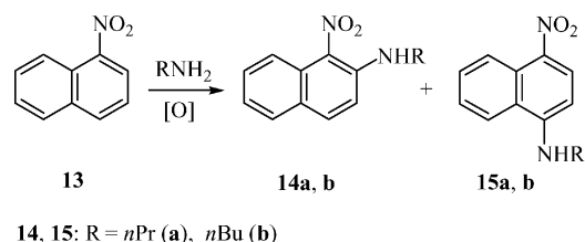
Scheme 5. Oxidative alkylamination of 1-nitronaphthalene (13).
