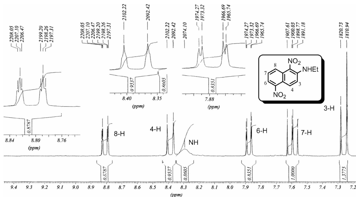
Figure 1. Fragment of the 1 H NMR spectrum of compound 5a (CDCl 3 ).
