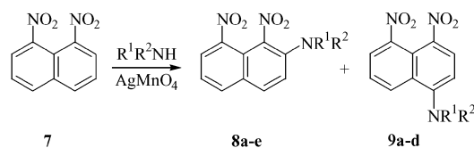
Scheme 4. Oxidative alkylamination of 1,8-dinitronaphthalene ( 7 ).
