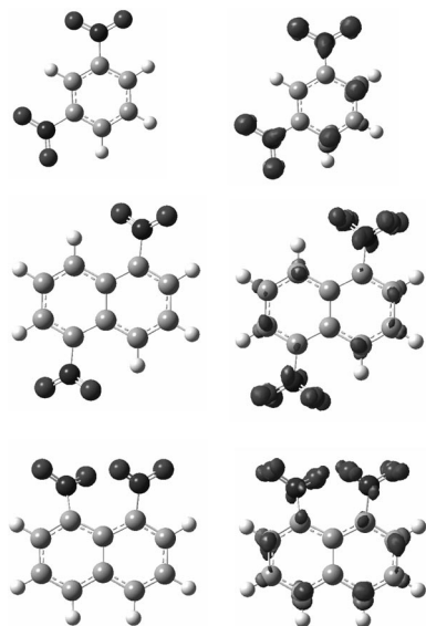
Figure 3. B3LYP/6-31G(d,p) equilibrium geometries (left) and corresponding Fukui functions (right) for nucleophilic attack on 1,3-dinitrobenzene (1, top), 1,5-dinitronaphthalene (4, middle), and 1,8-dinitronaphthalene (7, bottom). The values for the isodensity surfaces were set to 0.005 e a_0^{-3} .
